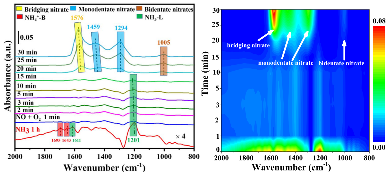
Fig. 10. In situ DRIFTS spectra of reaction between flue gases ( \text{NO} + \text{O}_2 ) and the preadsorbed \text{NH}_3 at 200 °C and the corresponding mapping results (right) over the Hierc- \text{MnFe}_{0.6}\text{Co}_{0.4}\text{O}_x catalyst.
