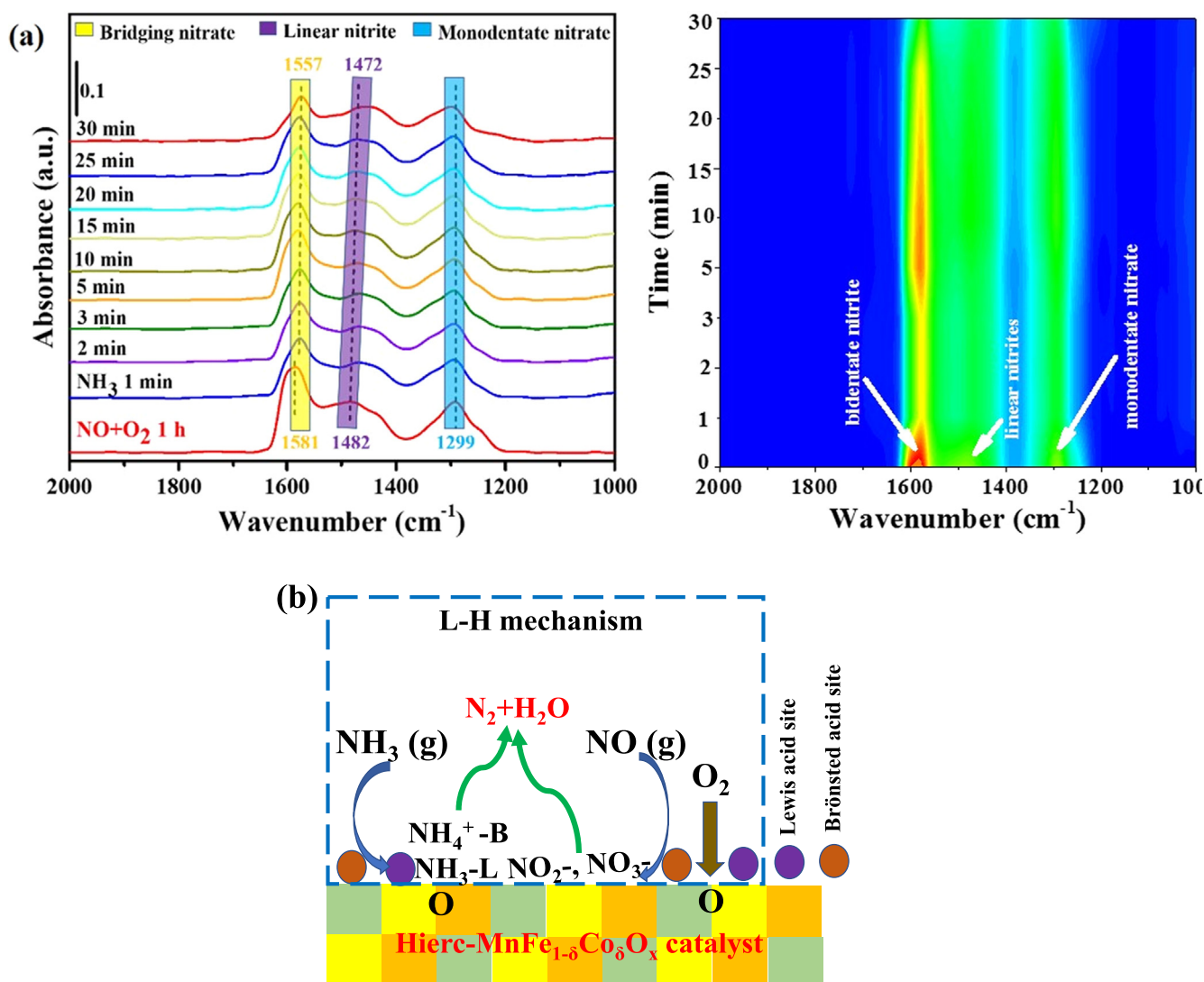
Fig. 11. (a) In situ DRIFTS spectra of reaction between \text{NH}_3 and preadsorbed \text{NO} + \text{O}_2 at 200 °C and the corresponding mapping results (right) over Hierc- \text{MnFe}_{0.6}\text{Co}_{0.4}\text{O}_x ; (b) proposed \text{NH}_3\text{-SCR} reaction mechanism over Hierc- \text{MnFe}_{0.6}\text{Co}_{0.4}\text{O}_x .
